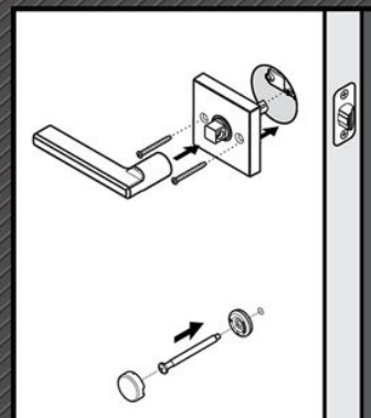
■ Install Interior Lever and Secure Handleset with Washer, Screw and Screw Cover
