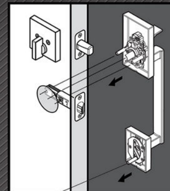
■ Place Handleset on Door; Requires Preexisting or New Hole Drilled Through Door
