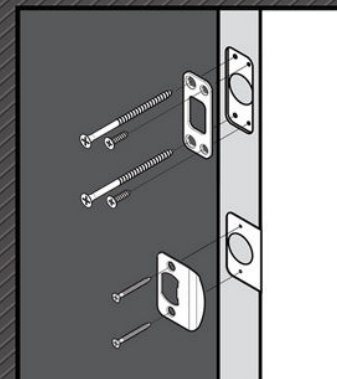
■ Install Top and Bottom Strikes
