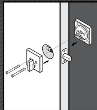
■ Place Deadbolt on Door and Secure with Screws
