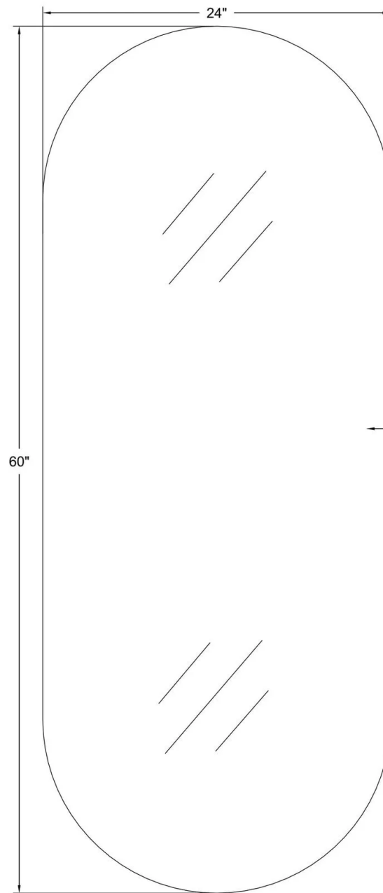
FRONT VIEW
