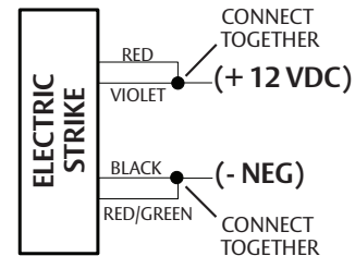
Diagram 1a: If Connector is Missing
