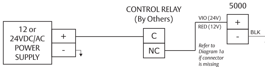
Diagram 3b: Fail Safe Wiring Example
