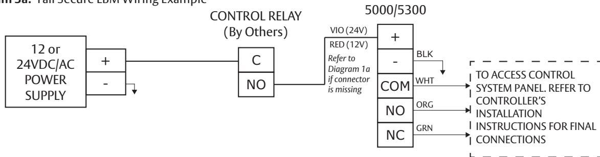
Diagram 3a: Fail Secure LBM Wiring Example
