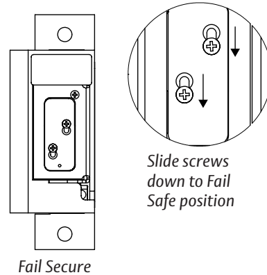
Diagram 2: Fail Safe Conversion
