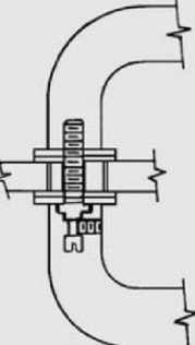
BACK TO BACK MTG. FOR GLASS DOORS C/W 1/8 x 1 1/4 WASHERS AND VINYL PADS FOR 3/8" - 1/2" GLASS STANDARD
