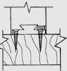
DOVETAIL CONCEALED MOUNTING
