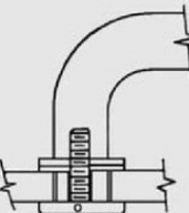
1 1/2" DIA. END CAP MOUNTING FOR 1/2" GLASS STANDARD C/W 1/8" x 1 1/4" - WASHERS
