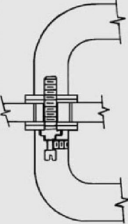
NO. 3-1 BACK TO BACK MTG FOR GLASS DOORS C/W 1/8 x 1 1/4 WASHERS AND VINYL PADS FOR 3/8" - 1/2" GLASS STANDARD
