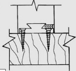
NO. 5 DOVETAIL CONCEALED MOUNTING
