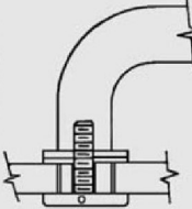
NO. 3-2 SINGLE CONCEALED MOUNTING FOR METAL DOORS REINFORCING HIGHLY RECOMMENDED
