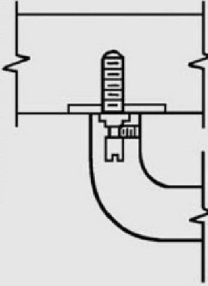
NO. 3-2 SINGLE CONCEALED MOUNTING FOR METAL DOORS REINFORCING HIGHLY RECOMMENDED
