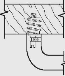
NO. 3-3 SINGLE CONCEALED MOUNTING FOR WOOD DOORS C/W STEEL INSERT
