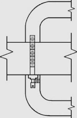
NO. 3 BACK TO BACK MTG FOR WOOD OR METAL DOORS 1 3/4" STANDARD
