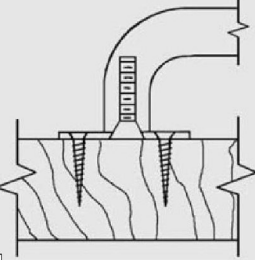
NO. 4 SURFACE MOUNTING
