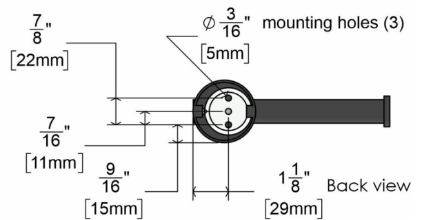
3d Back view - assembly
