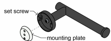
3d Back view - assembly
